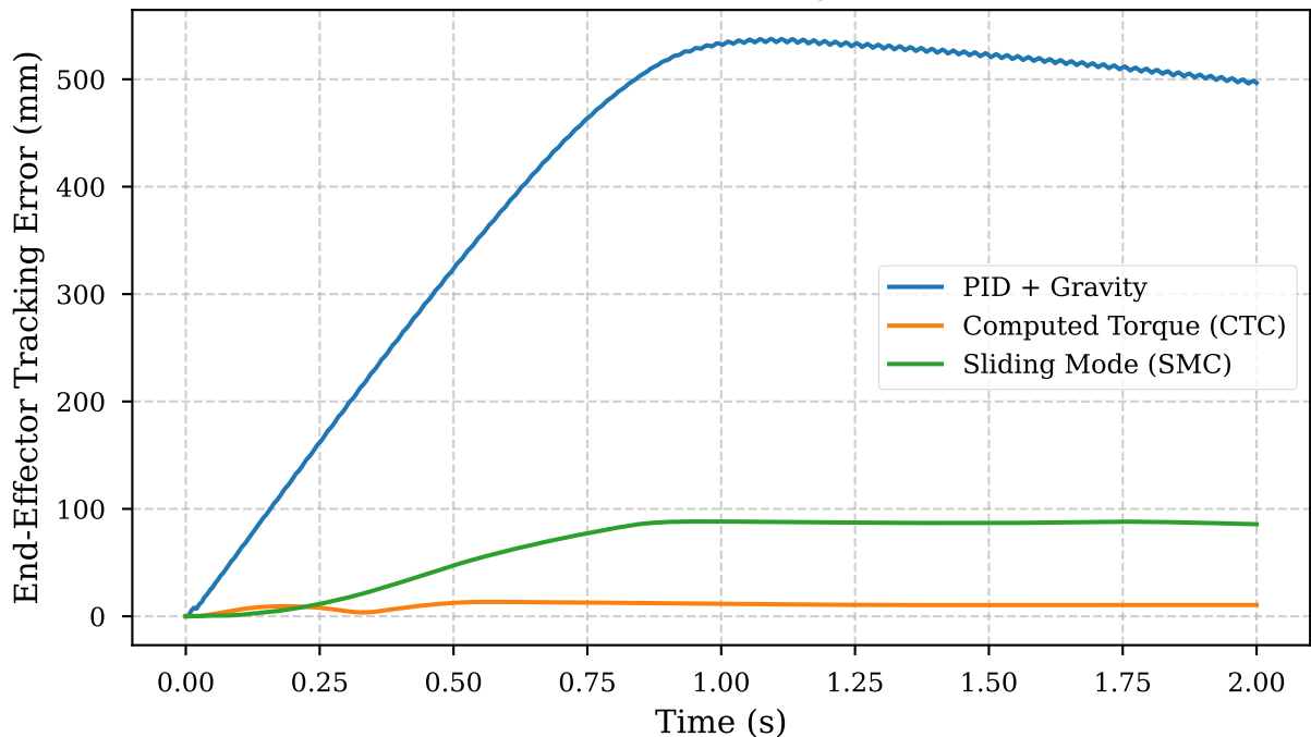
End-Effector Spatial Position Tracking Error Under Disturbance
